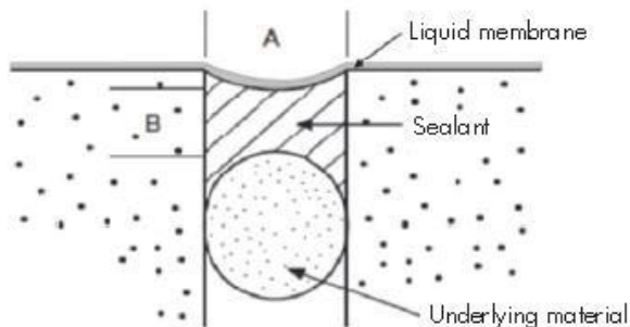
Correctly dimensioned joint A:B=2:1, dimension A,B min. 6mm
