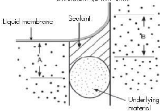
Correctly executed angle joint dimension A,B min. 6mm
